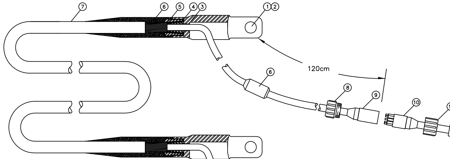
10 PIN INSERT, EXTERIOR VIEW
